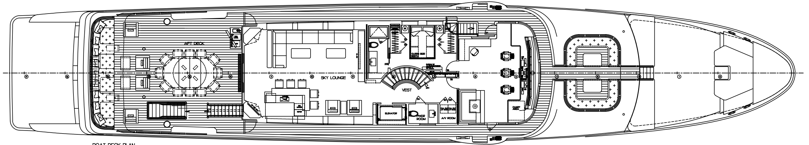
BOAT DECK PLAN
